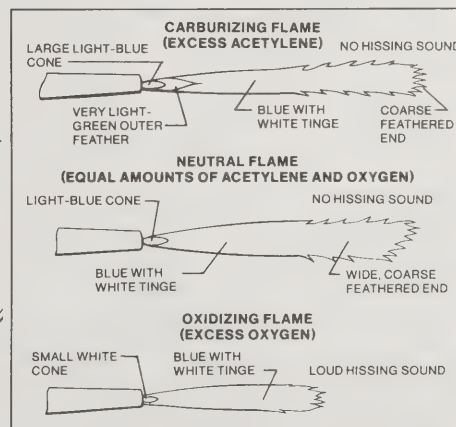
Basic gas-welding flames: Each has distinctive shape, color and sound. Neutral flame is the most used.
